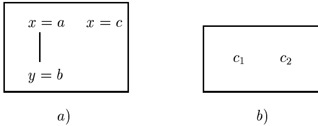
Fig. 1. Partial orders.
