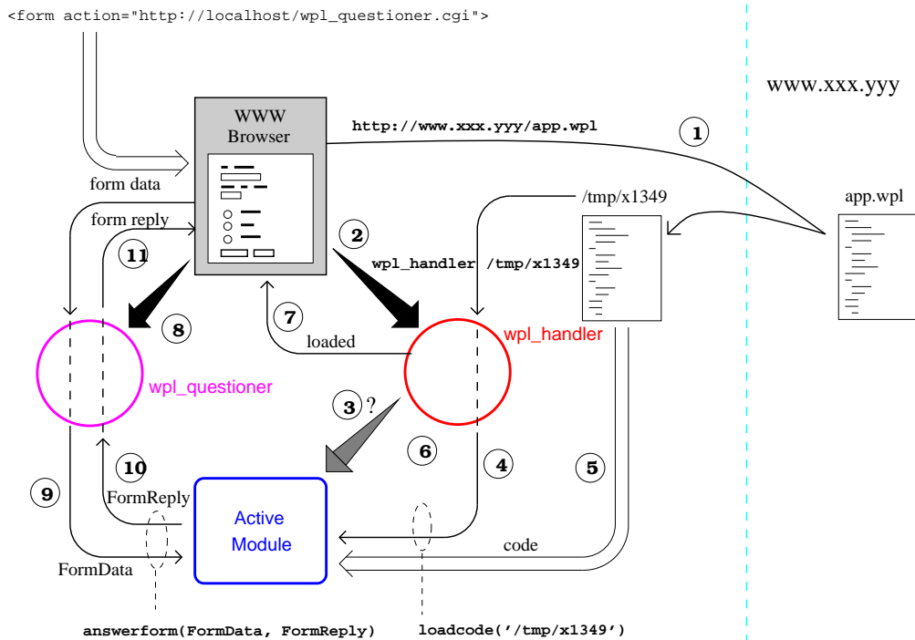
Figure 4: Automatic code downloading architecture
