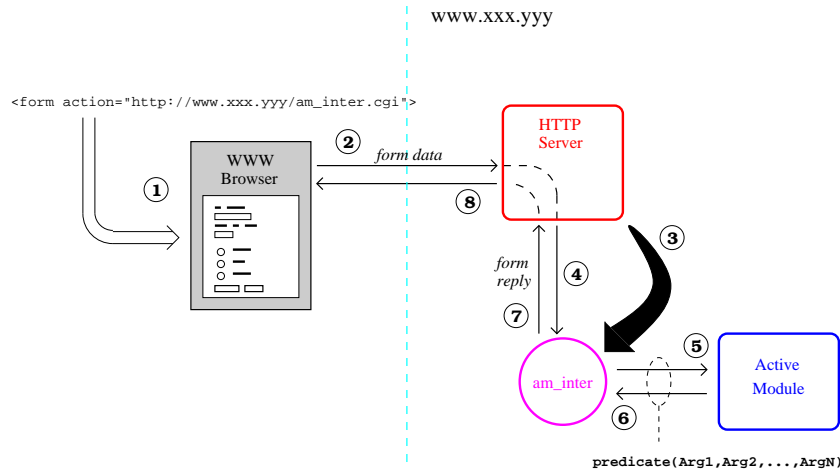
Figure 3: The Forms Interface using Active Modules
