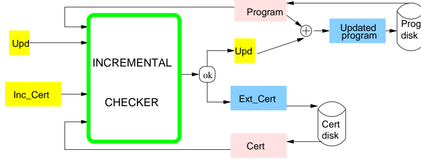
Fig. 2. Incremental Checking in Abstraction-Carrying Code
