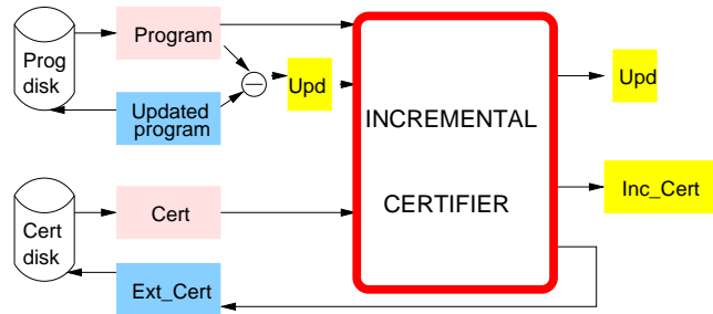
Fig. 1. Incremental Certification in Abstraction-Carrying Code
