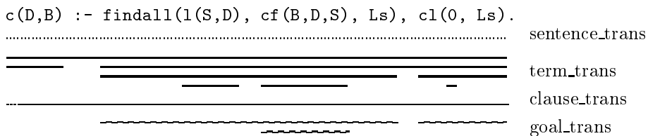
Figure 1: Subterms to which each translation type is applied in a clause
