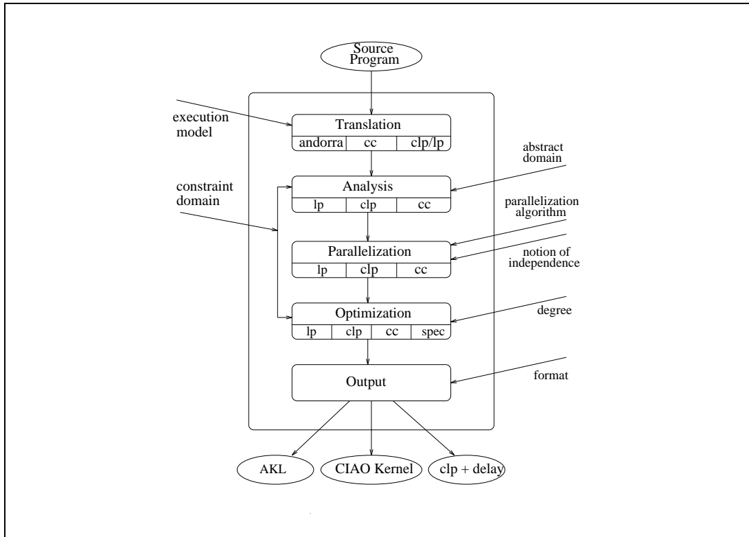
Figure 1: CIAO Compiler
