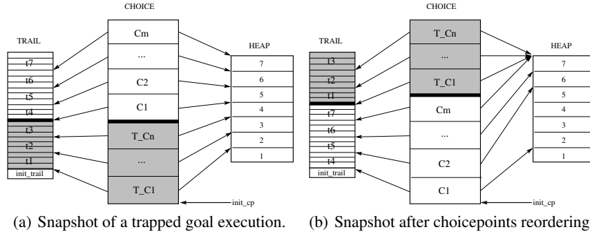
Fig. 2. Example of choicepoint reordering before executing a trapped goal.
