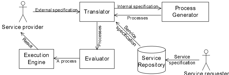
Fig. 1. The framework of the service composition system
