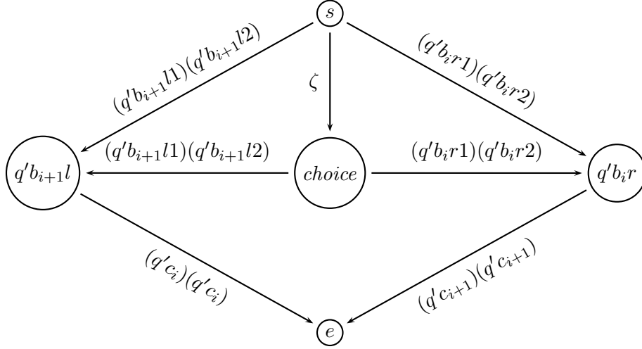
Figure 4: Automaton K
