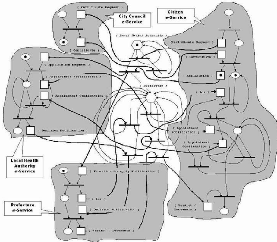
Fig. 3. The orchestration schema ( E -service and Orchestration Nets) of the running example
