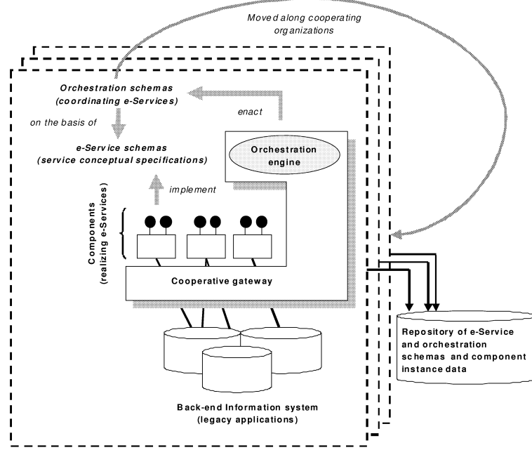
Fig. 1. The PARIDE framework
