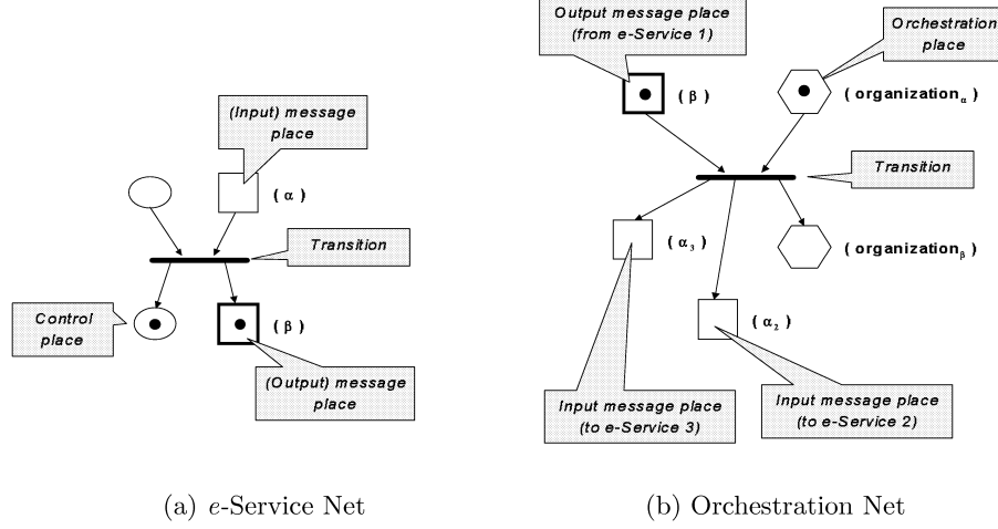
Fig. 2. Basic elements of the Petri Net-based model
