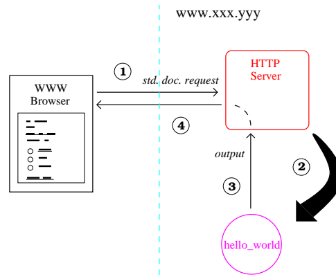
Fig. 1. The CGI interface
