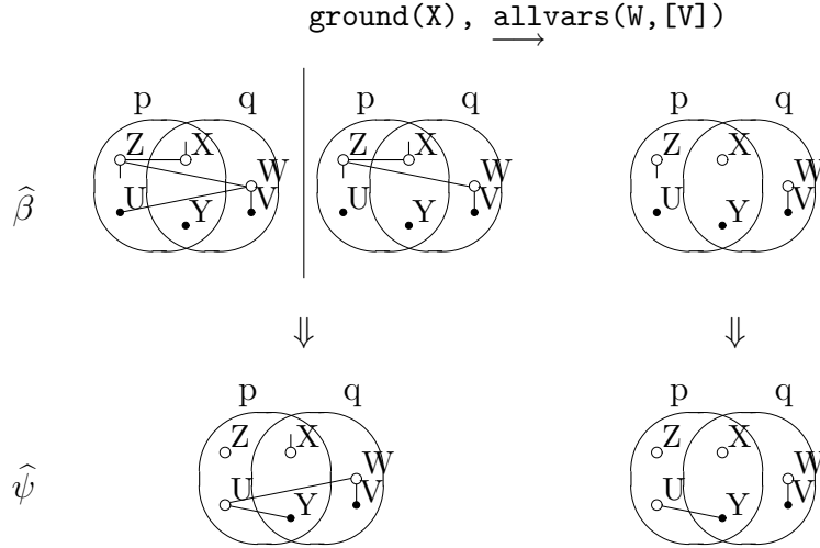
Fig. 6. Restriction of the possible sharing sets by the checks make the goals non-strictly independent.
