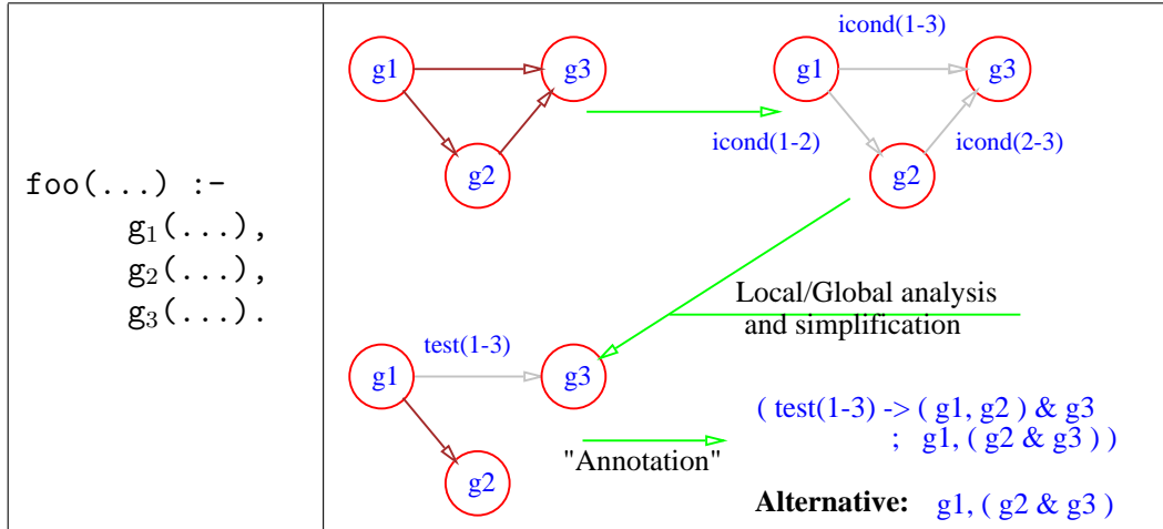
Fig. 1. Parallelizing “ g_1(\dots) , g_2(\dots) , g_3(\dots) ” in \& -Prolog/CiaoPP
