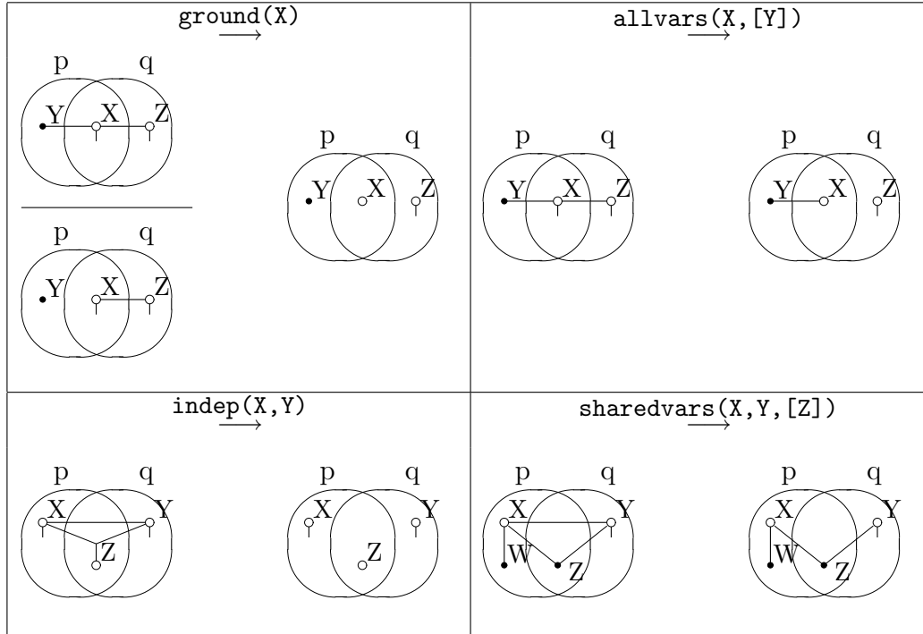
Fig. 5. Example applications of the four checks.
