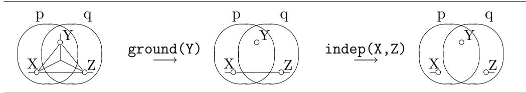
Fig. 7. Restriction of the possible sharing sets performed by the checks.
