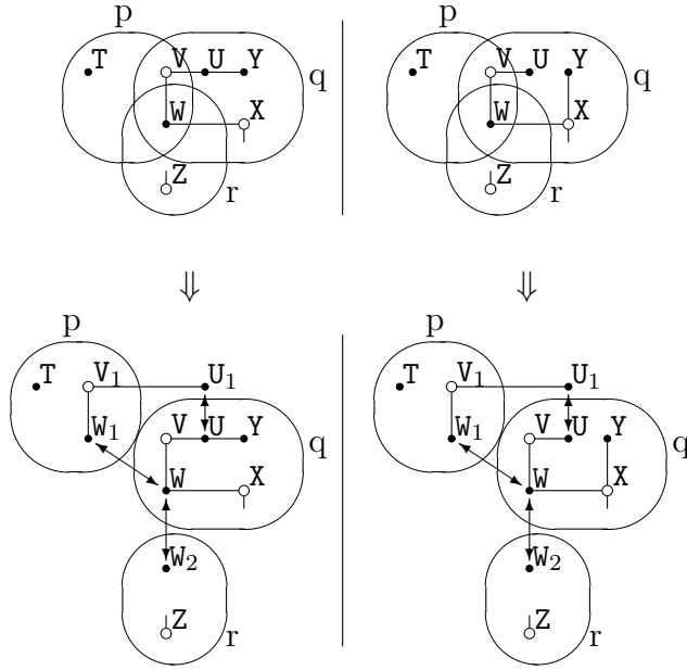
Fig. 12. Representation of the effect of variable replacement in a parallel expression.
