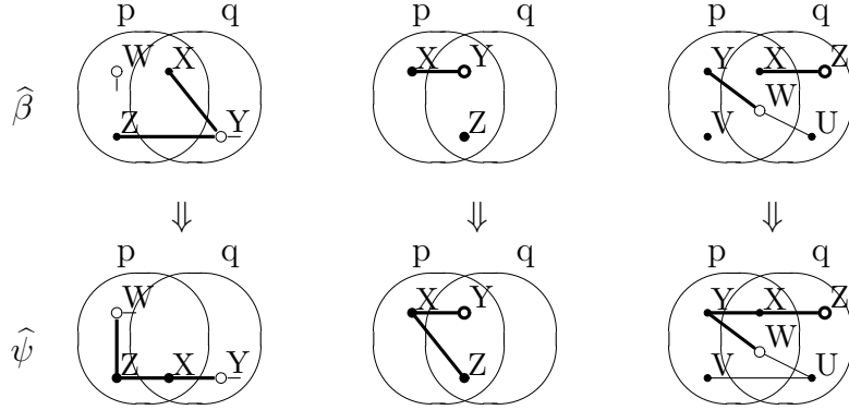
Fig. 4. Situations where the conditions do not hold, and thus the goals are possibly not non-strictly independent.
