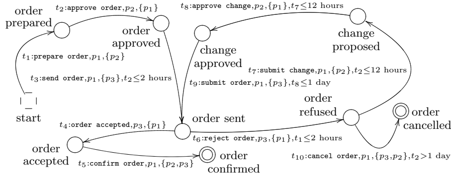
Fig. 1. The Purchase Order business protocol.
